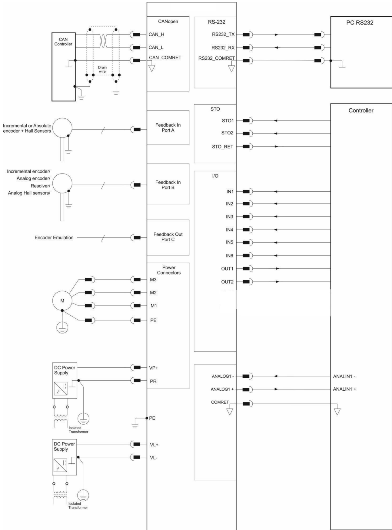
Figure 2: The Gold DBWhistle CAN Connection Diagram
