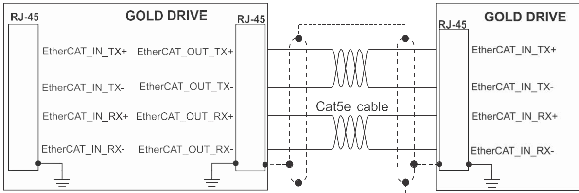
Figure 17: EtherCAT RJ-45 Connections
