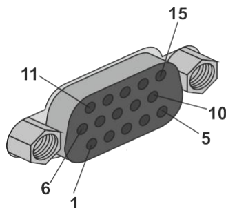
15-Pin D-Type Female Connector
