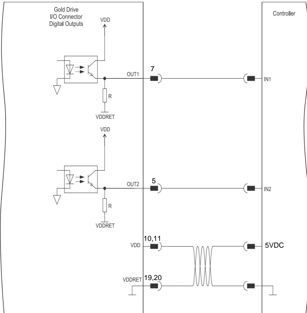
Figure 19: Digital Output Connection Diagram Example – Source 5V Logic Option
