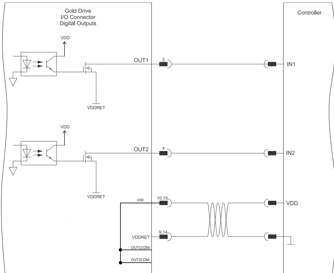
Figure 18: Digital Output Connection Diagram Example – NPN
