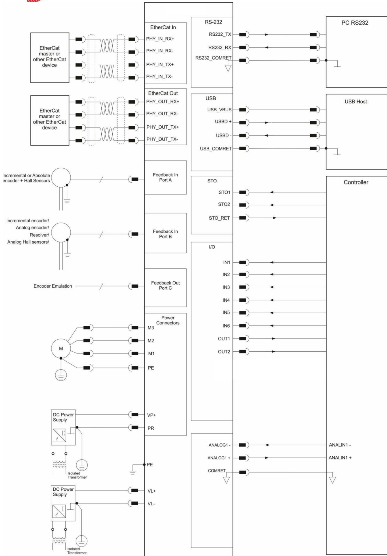
Figure 3: The Gold DBWhistle EtherCAT Connection Diagram
