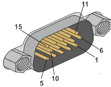
15-Pin D-Type Female Connector
