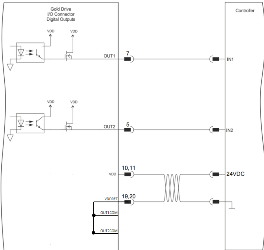
Figure 17: Digital Output Connection Diagram Example – PNP
